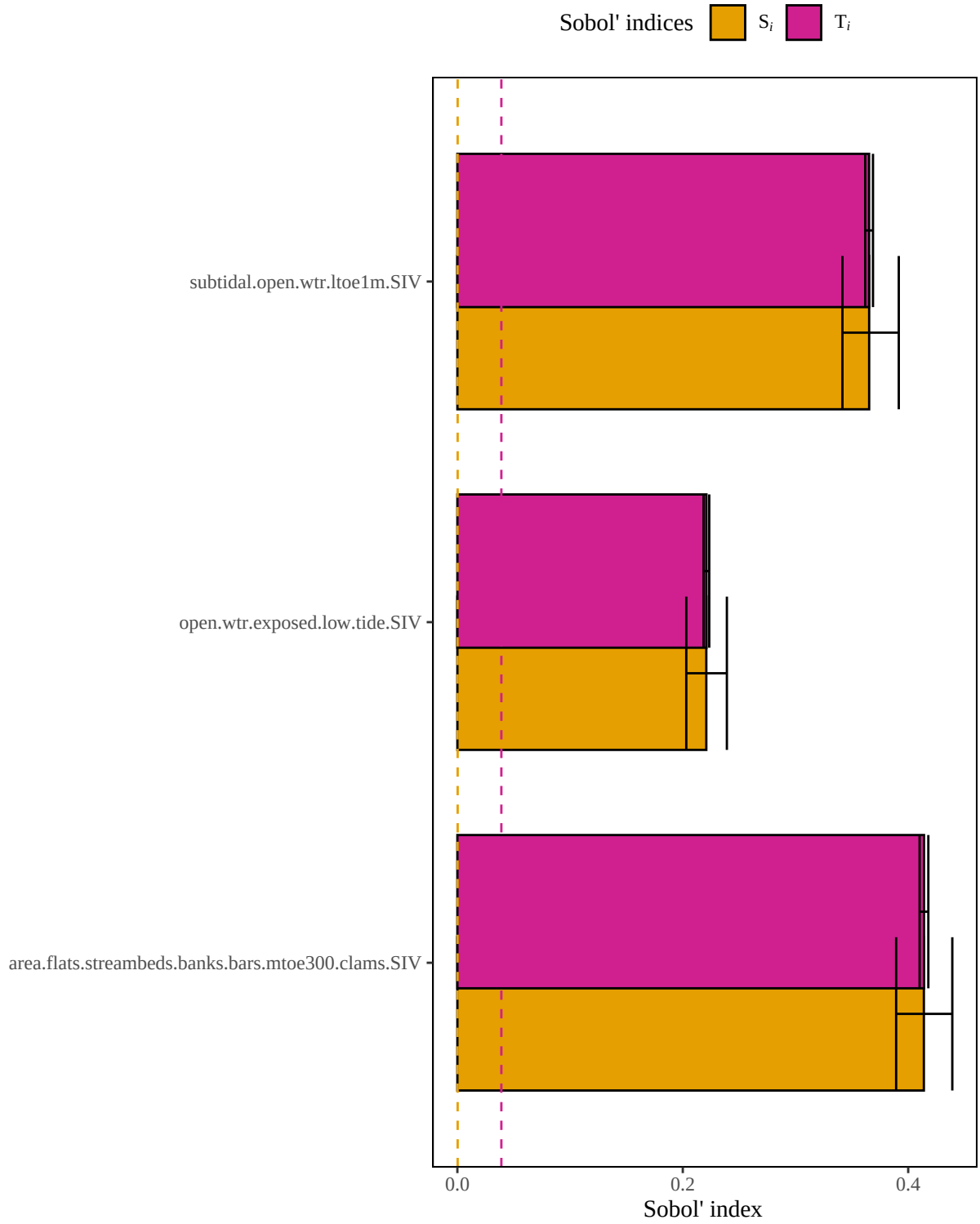
Figure 4. Results of a sensitivity analysis for the americanblackduckWinteringNCapeCod model based on an arithmetic mean structure. Dashed lines represent baseline numerical approximation error for S_i and T_i ( i.e. , dummy variables).
